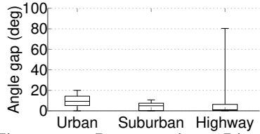
Figure 16: 3D ray-tracing - Distribution of angle gaps between recoverable paths AoD and last LoS AoD.
