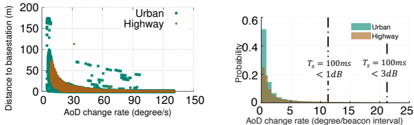
Figure 11: 3D ray-tracing - AoD changes v.s. distance to basestation. Figure 12: 3D ray-tracing - AoD changes histogram.
