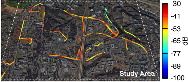
Figure 6: 3D ray-tracing - Large scale coverage heatmap of co-locating mmWave basestations with LTE basestations.
