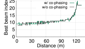
Figure 23: Measurement - Best beam index dynamics.
