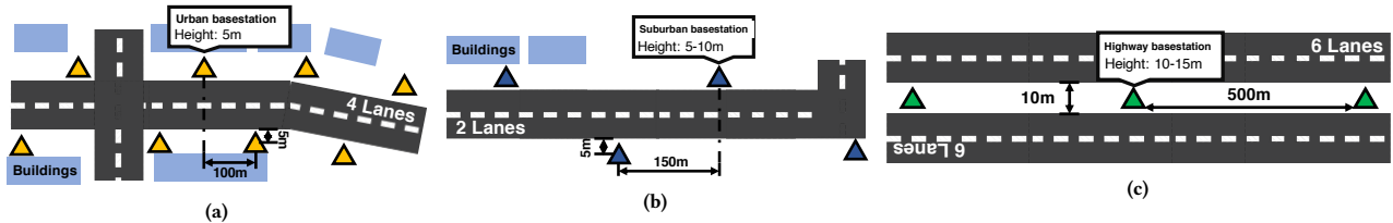
Figure 4: Scenario-specific 3D ray-tracing basestation deployment of (a) Urban, (b) Suburban, (c) Highway.
