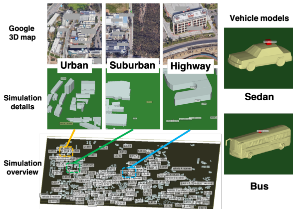
Figure 3: Large-scale 3D ray-tracing overview.
