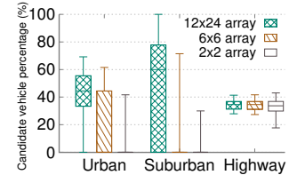
Figure 26: 3D ray-tracing - Opportunities for spatial-orthogonal multiplexing.
