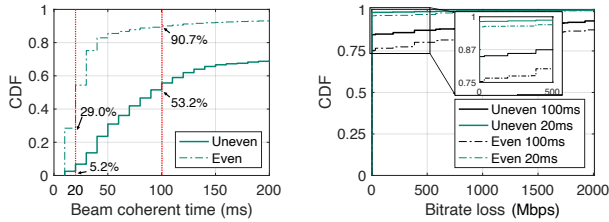
Figure 14: 3D ray-tracing - Beam coherent time comparison of two codebooks. Figure 15: 3D ray-tracing - Bitrate loss comparison of two codebooks.
