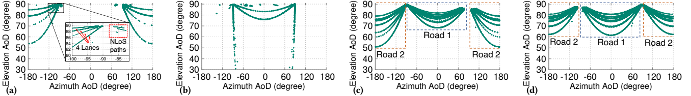
Figure 9: 3D ray-tracing - AoD distribution showcases (a) Urban basestation 1. (b) Urban basestation 2. (c) Highway basestation 1. (d) Highway basestation 2.
