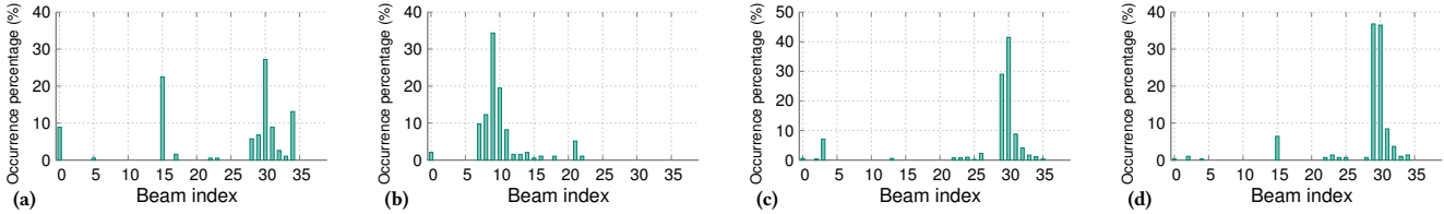
Figure 8: Measurement - Best beam histogram of 4 testbed basestations: (a)RSU1, (b)RSU2, (3)RSU3, (4)RSU4.
